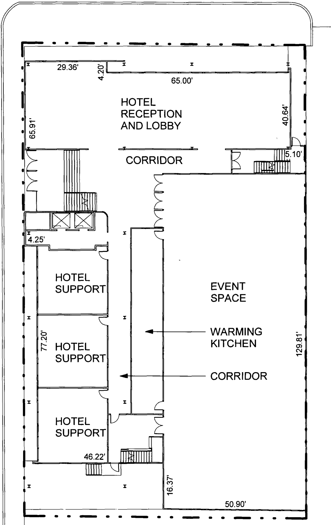
① ZN - FIRST FLOOR PLAN 3/64" = 1'-0"
