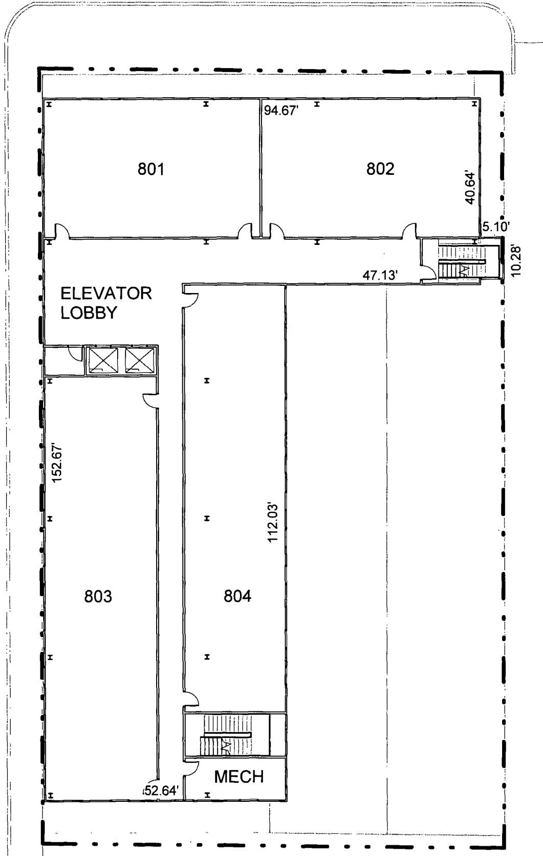
① ZN - EIGHTH FLOOR PLAN 3/64" = 1'-0"
