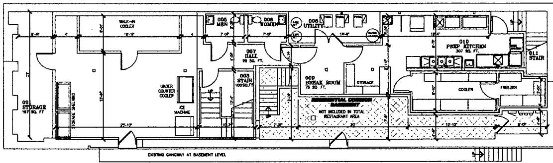
First Floor Occupancy Plan Scale: 1/4" = 1'
