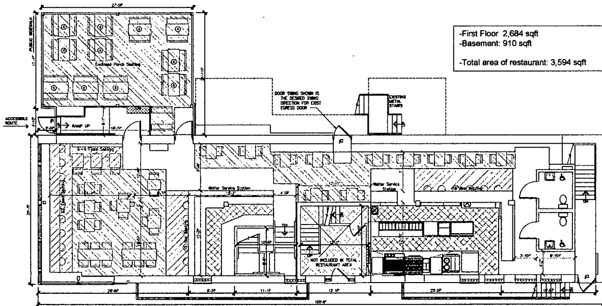
First Floor Occupancy Plan Scale: 1/4" = 1'
