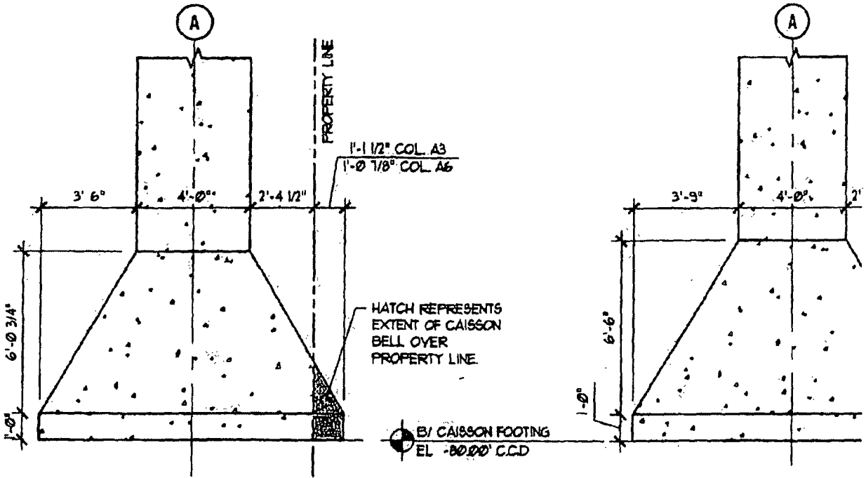
① 11' 0" DIA BELL DETAIL SCALE 1/4" = 1' 0"
