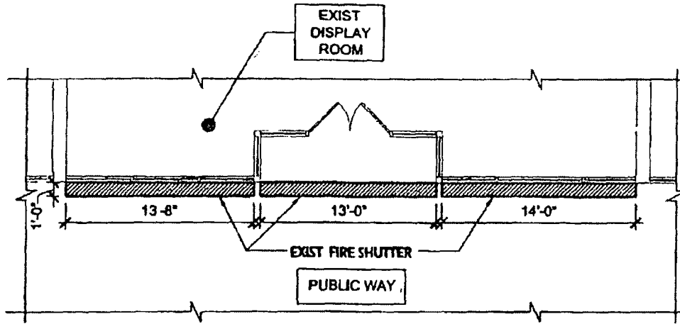
EXIST FIRE SHUTTER LAYOUT SCALE 1/8" = 1'-0"
