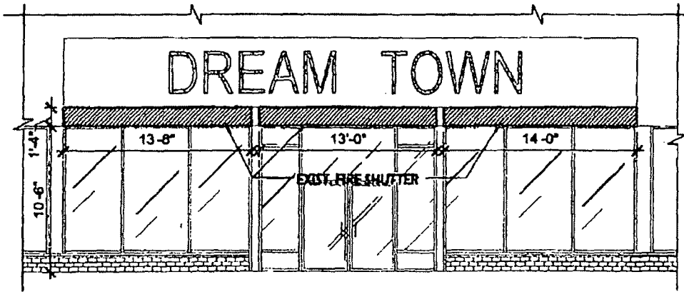
EXIST. FRONT ELEVATION SCALE 1/8" = 1'-0"
