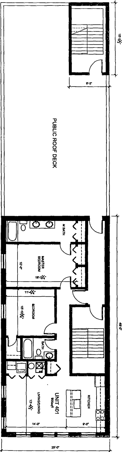
FOURTH FLOOR/ROOF DECK PLAN SCALE: \frac{1}{8}''=1'-0''
