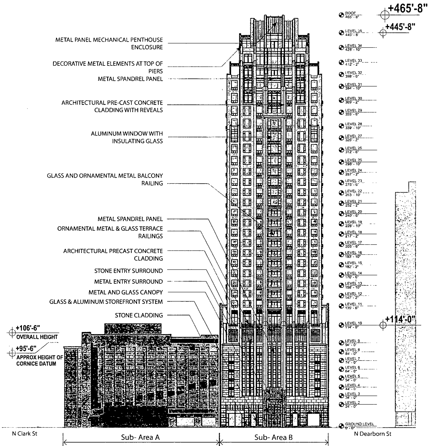
SOUTH ELEVATION
