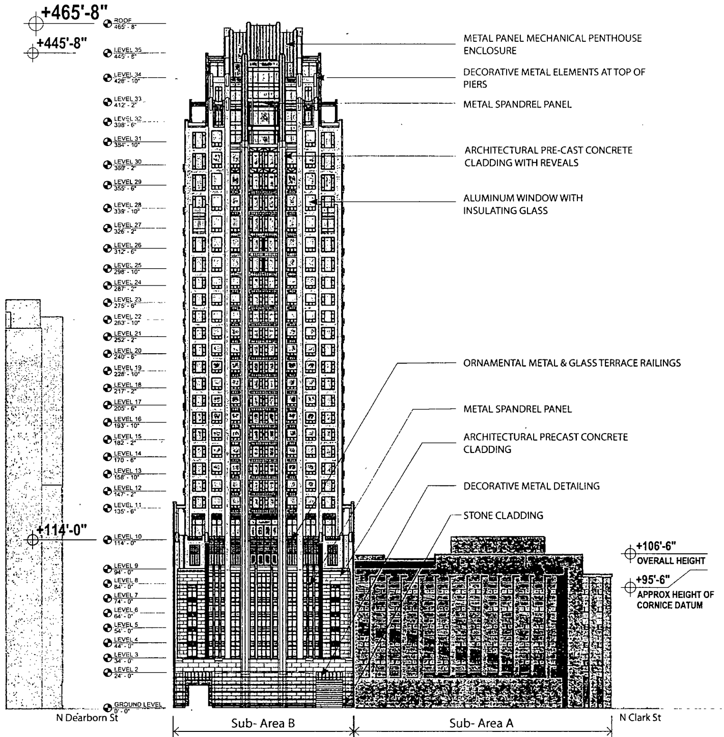
NORTH ELEVATION
