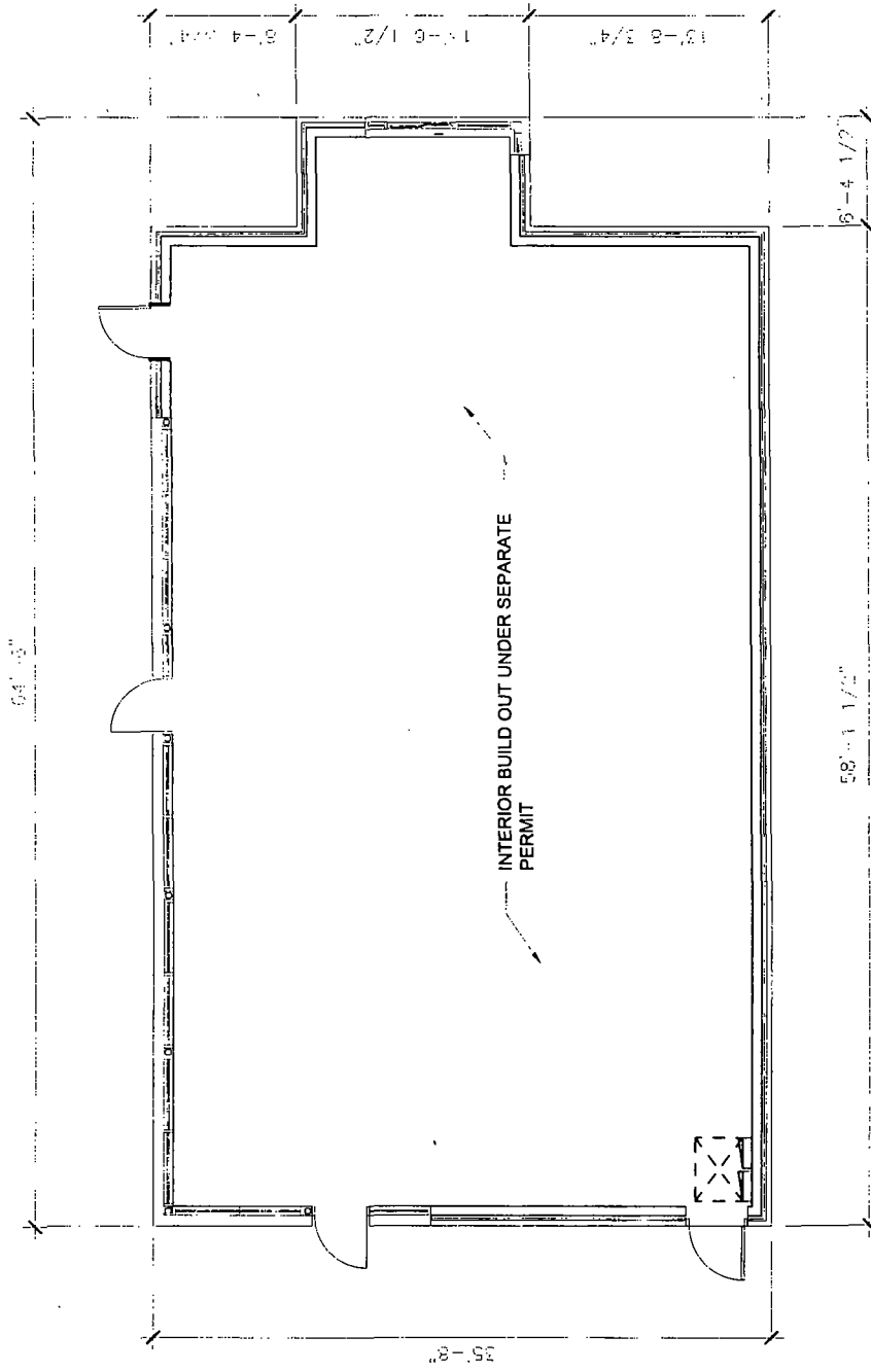
1 FLOOR PLAN SCALE 3/32"=1'-0"
