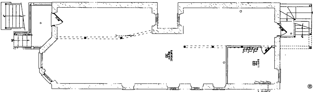
0 BASEMENT PLAN SCALE 1/8" = 1'-0"
