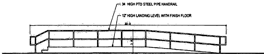
ELEVATION OF RAMP, STEPS, LANDING AND HANDRAIL IN PUBLIC WAY
