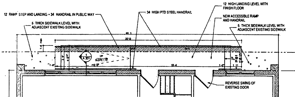
PLAN OF RAMP, STEPS, LANDING AND HANDRAIL IN PUBLIC WAY
