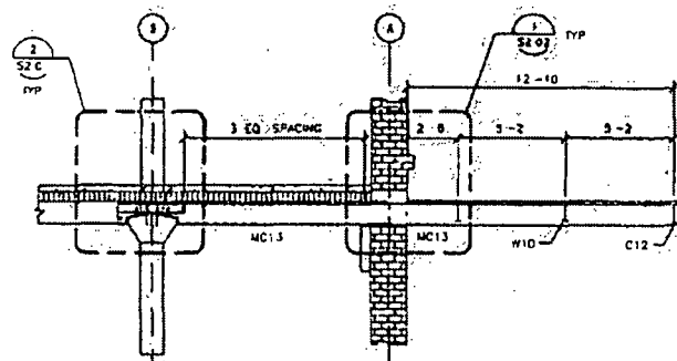
3 | CANOPY SECTION AT COL LINE 22
