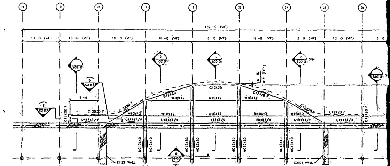
1 | CANOPY FRAMING PLAN
