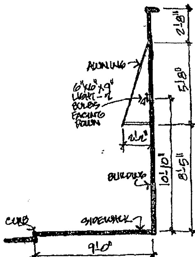
SECTION & AWNING
