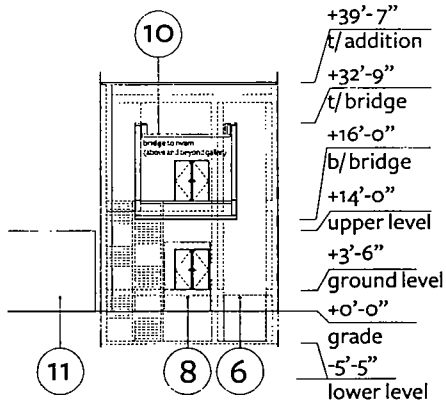
I. NORTH ELEVATION - NVAM
