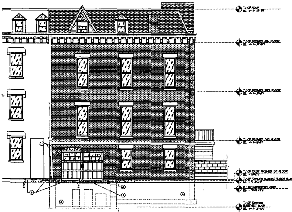
PROPOSED WEST ELEVATION 1
