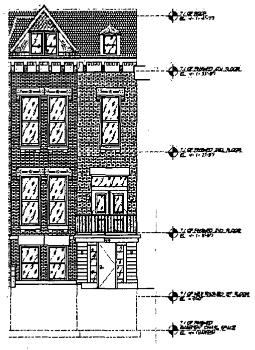
EXISTING SOUTH ELEVATION 3
