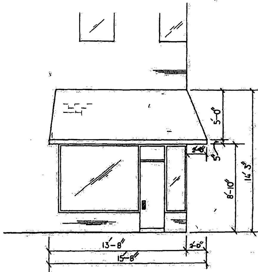
EAST ELEVATION
