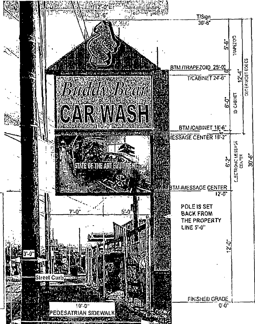
Proposed Business Pole Sign Rendering SCALE: 3/16" = 1'-0"
