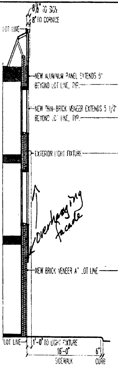
West Wall Section 1/8" = 1'-0"
