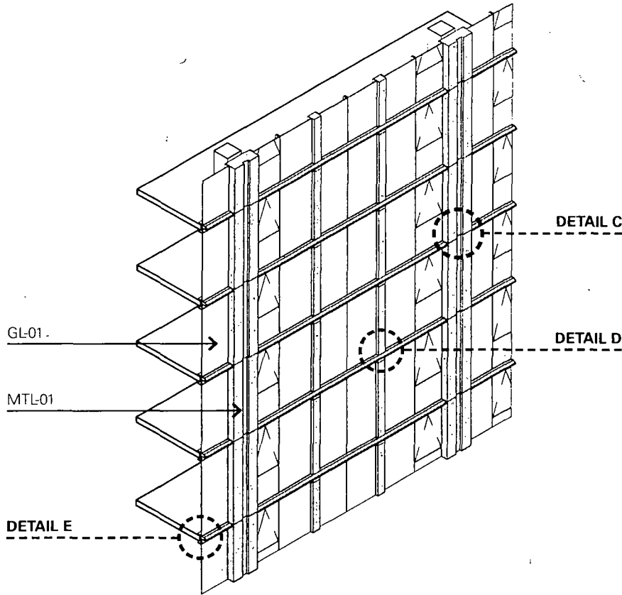
EAST ELEVATION
